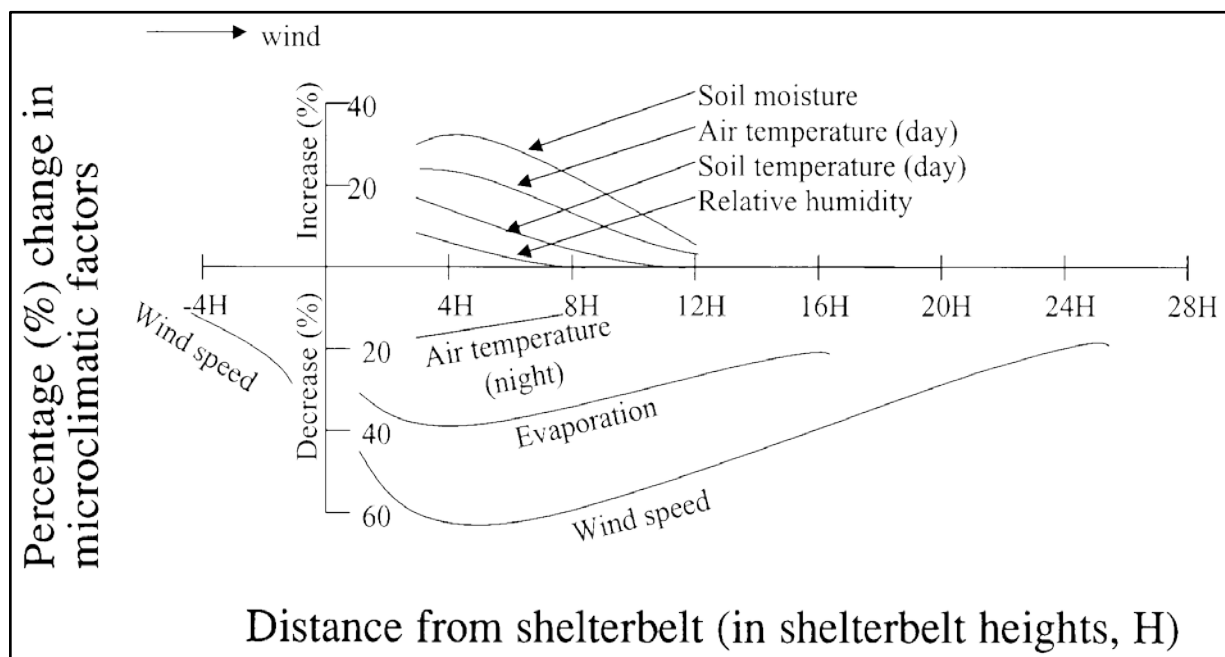
Figure 1: The effect of a shelterbelt on microclimate (modified from Marshall 1967)
